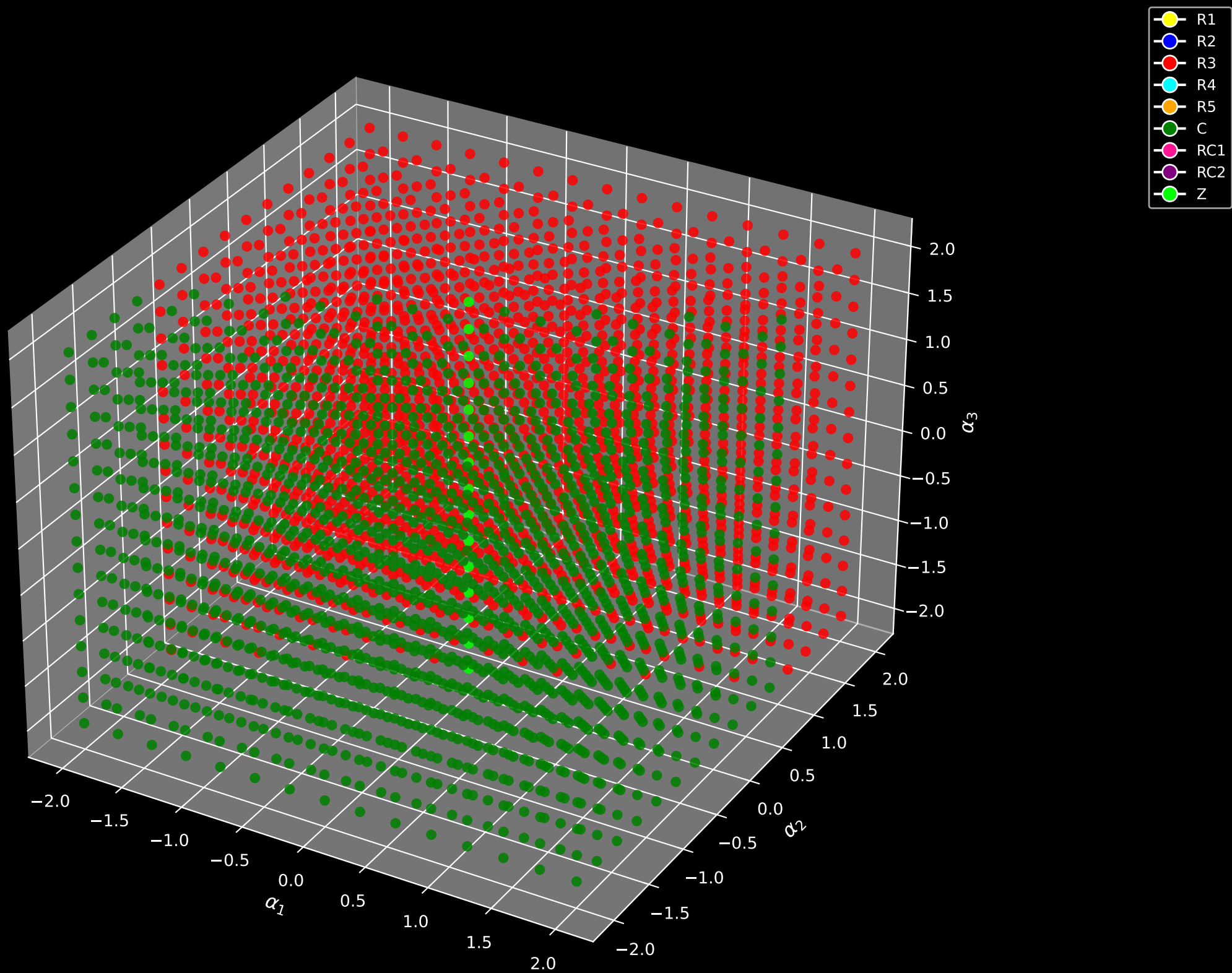
Eigenvalue Categorization (Fixed \alpha_4 = -0.80 )
