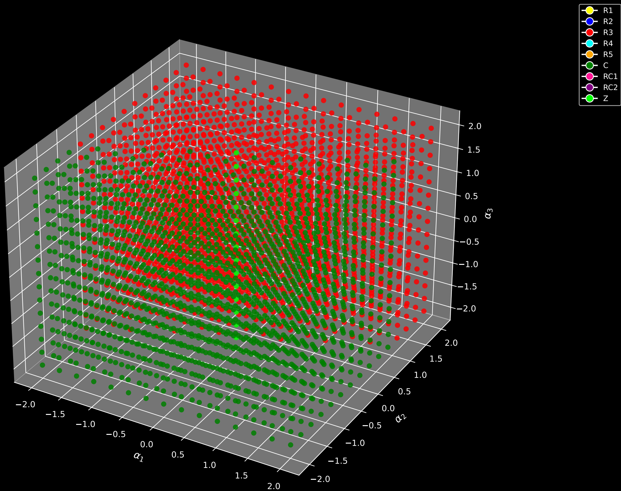
Eigenvalue Categorization (Fixed \alpha_4 = -1.10 )
