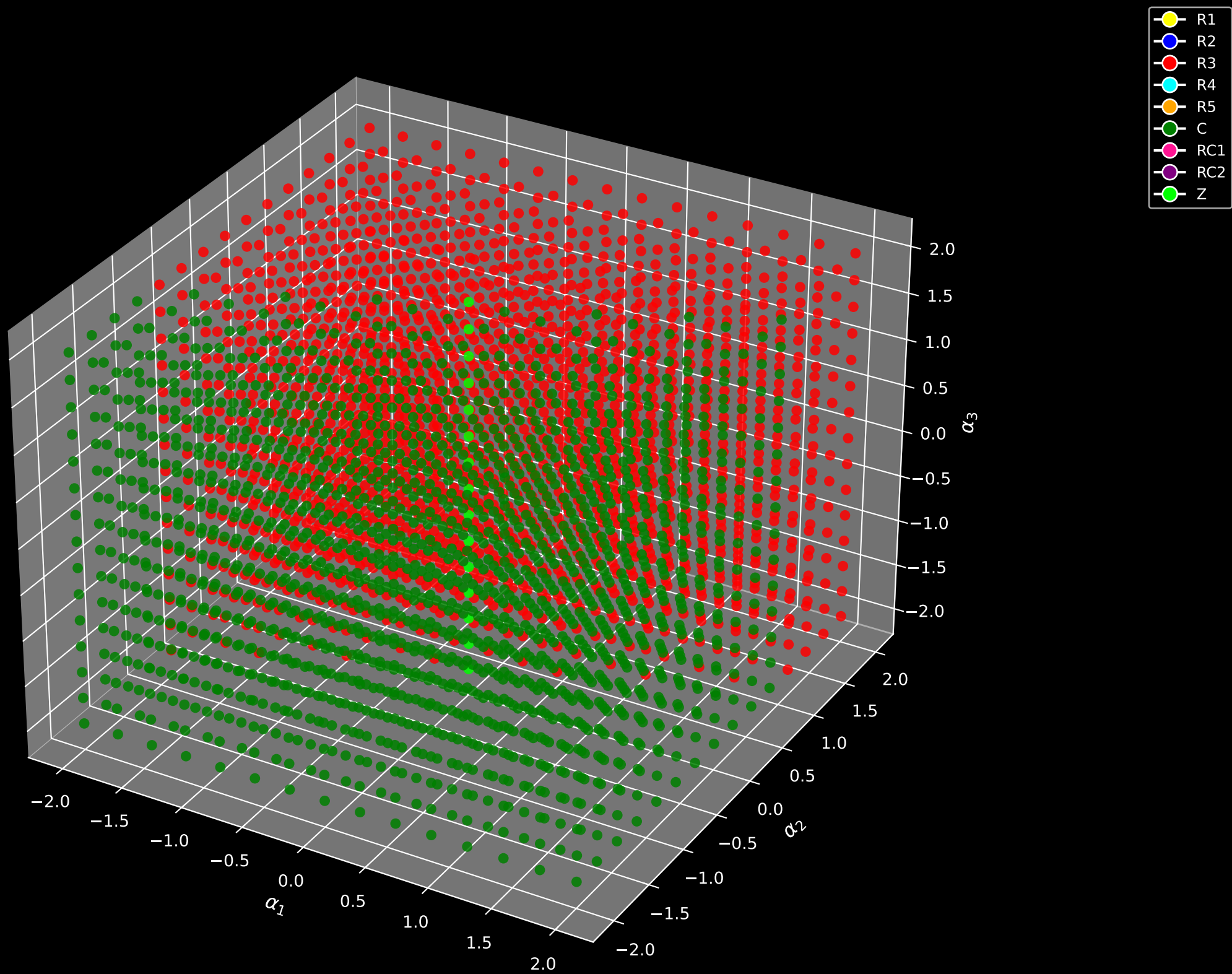
Eigenvalue Categorization (Fixed \alpha_4 = -1.70 )
