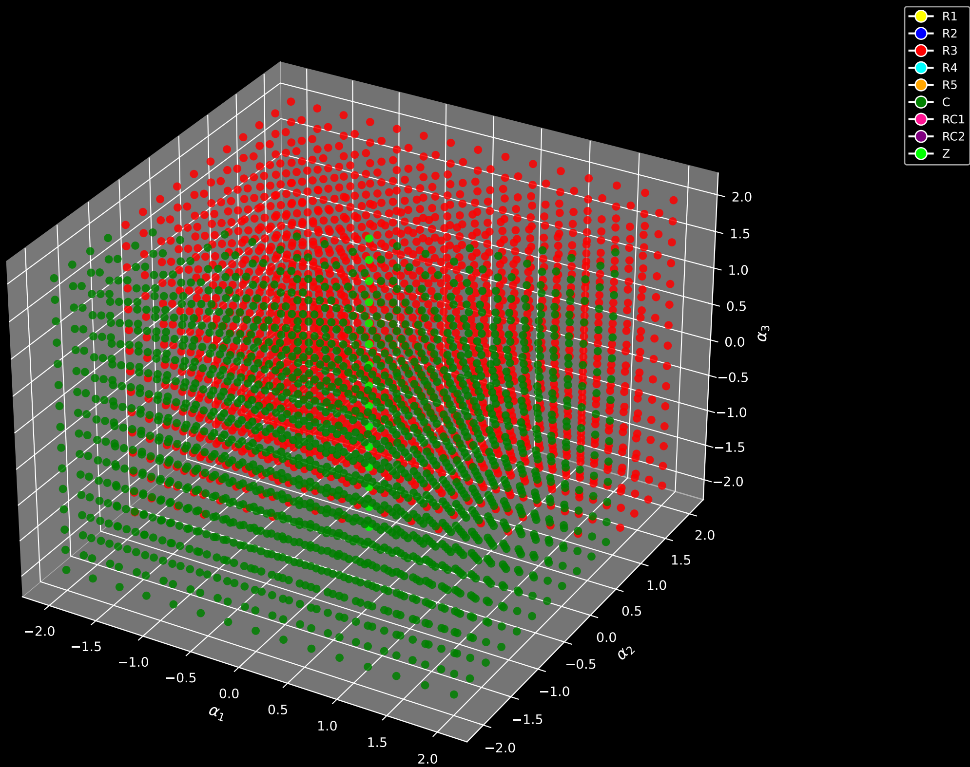
Eigenvalue Categorization (Fixed \alpha_4 = 1.90 )
